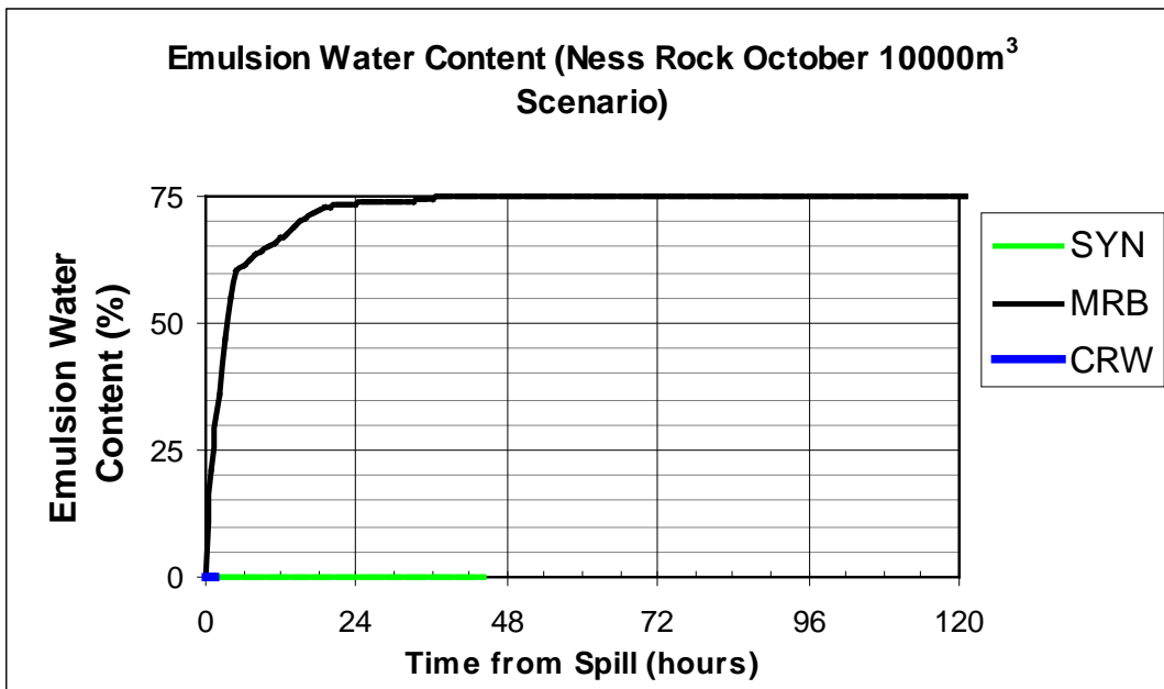
Figure 2-36 Emulsion Water Content (Ness Rock October 10,000 m 3 Scenario)
